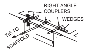
SECURE AT WINDOW OPENING
