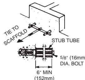
SECURE TO EMBEDDED TIES IN CONCRETE
