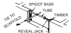
SECURE TO REVEAL PROP. fig. D
